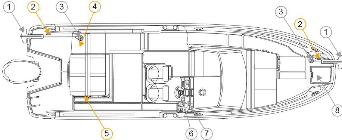
Figure 4.11 Anchor windlass
